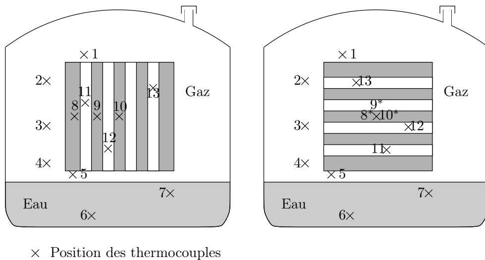
Cube aux perforations verticales Cube aux perforations horizontales
